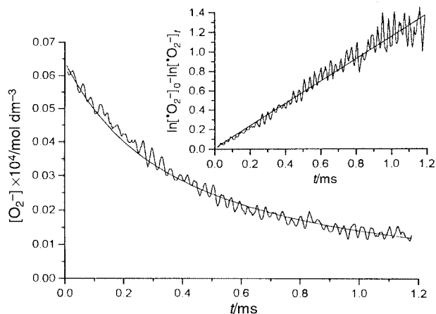
Fig. 7 Typical kinetic plot describing the decay of absorbance of ^{\circ}\text{O}_2^- at 250 \text{ nm} in an \text{O}_2 -saturated solution containing 1.32 \times 10^{-5} \text{ mol dm}^{-3} \text{Cu}(\text{ClO}_4)_2 , 9.12 \times 10^{-6} \text{ mol dm}^{-3} ligand and 0.10 \text{ mol dm}^{-3} sodium formate at \text{pH } 7.4 . Inset: plot of \ln[^{\circ}\text{O}_2^-]_0 - \ln[^{\circ}\text{O}_2^-]_t vs. t . The broken line denotes the experimental data (355 points were recorded) and the smooth curve denotes the fitted line.
