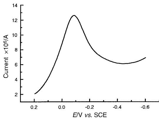
Fig. 6 Differential-pulse voltammogram profile of a solution containing 1 \times 10^{-3} \text{ mol dm}^{-3} complex (initial E = 0.2 \text{ V} , final E = -0.6 \text{ V} , increment in E = 0.04 \text{ V} , amplitude = 0.05 \text{ V} , pulse width = 0.06 \text{ s} , sample width = 0.02 \text{ s} , pulse period = 0.2 \text{ s} ).
